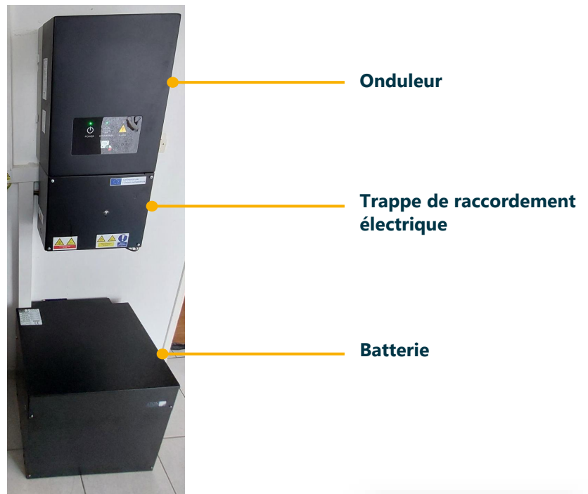
Armoire H-STORE
